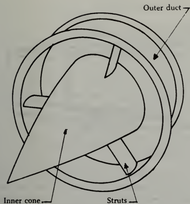
FIGURE 1-61. Exhaust collector with welded support struts.
